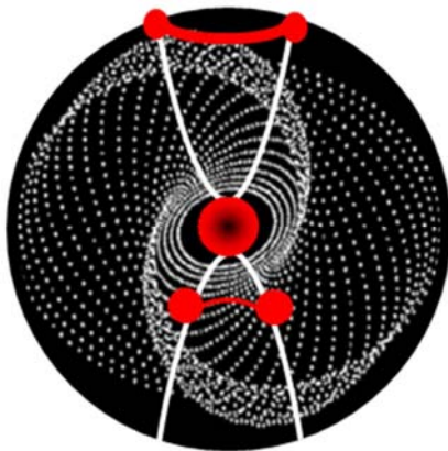
Figure 10. All these variables help to create shapes in galaxies like the golden spiral (φ = 1,6180).
